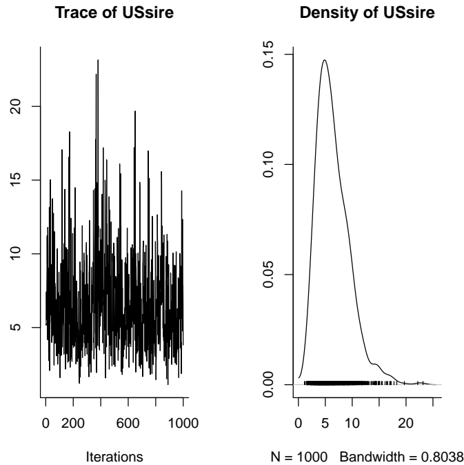
Figure 9: The marginal posterior distribution of the number of unsampled males from model16 . In this model an informative prior was used.
