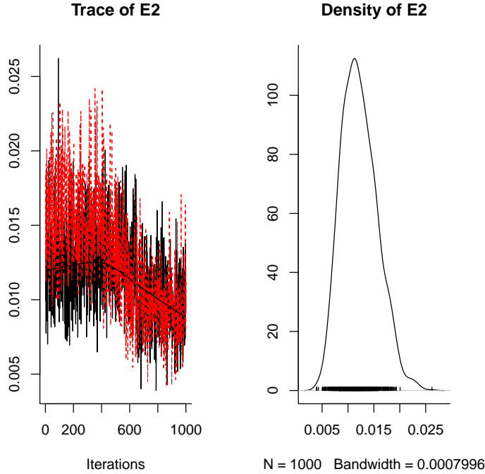
Figure 12: Samples from the posterior distribution of stochastic error rate estimated from the data set Gobs . The two chains were initialised at the true genotype configuration (black), and a random configuration (red).
