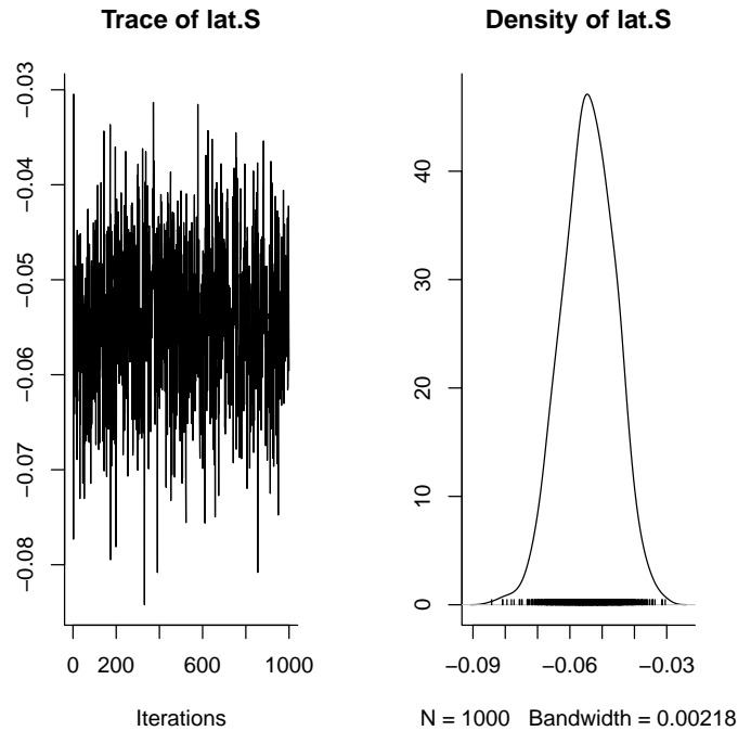
Figure 5: Posterior distribution of \beta from model2 . The posterior is conditional on the categorical assignment of the pedigree being true. These plots are a way of summarising a Markov Chain using the coda package. The left plot is a trace of the sampled posterior, and can be thought of as a time series. The right plot is a density estimate, and can be thought of a smoothed histogram approximating the posterior. See Section 1 for more details.
